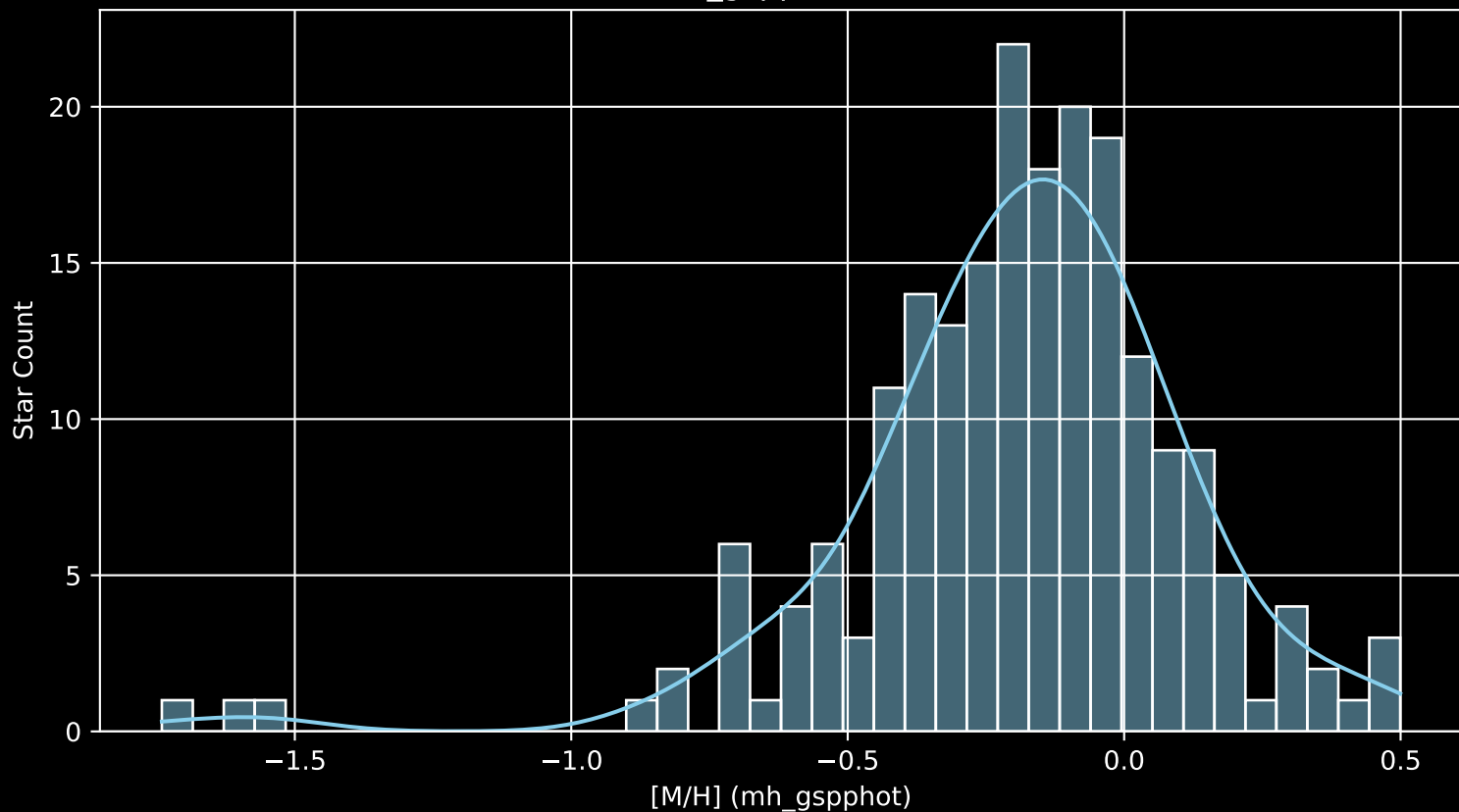
APOGEE DR17 Field: [163+36_MGA [M/H] (mh_gspphot) (n= 204)
