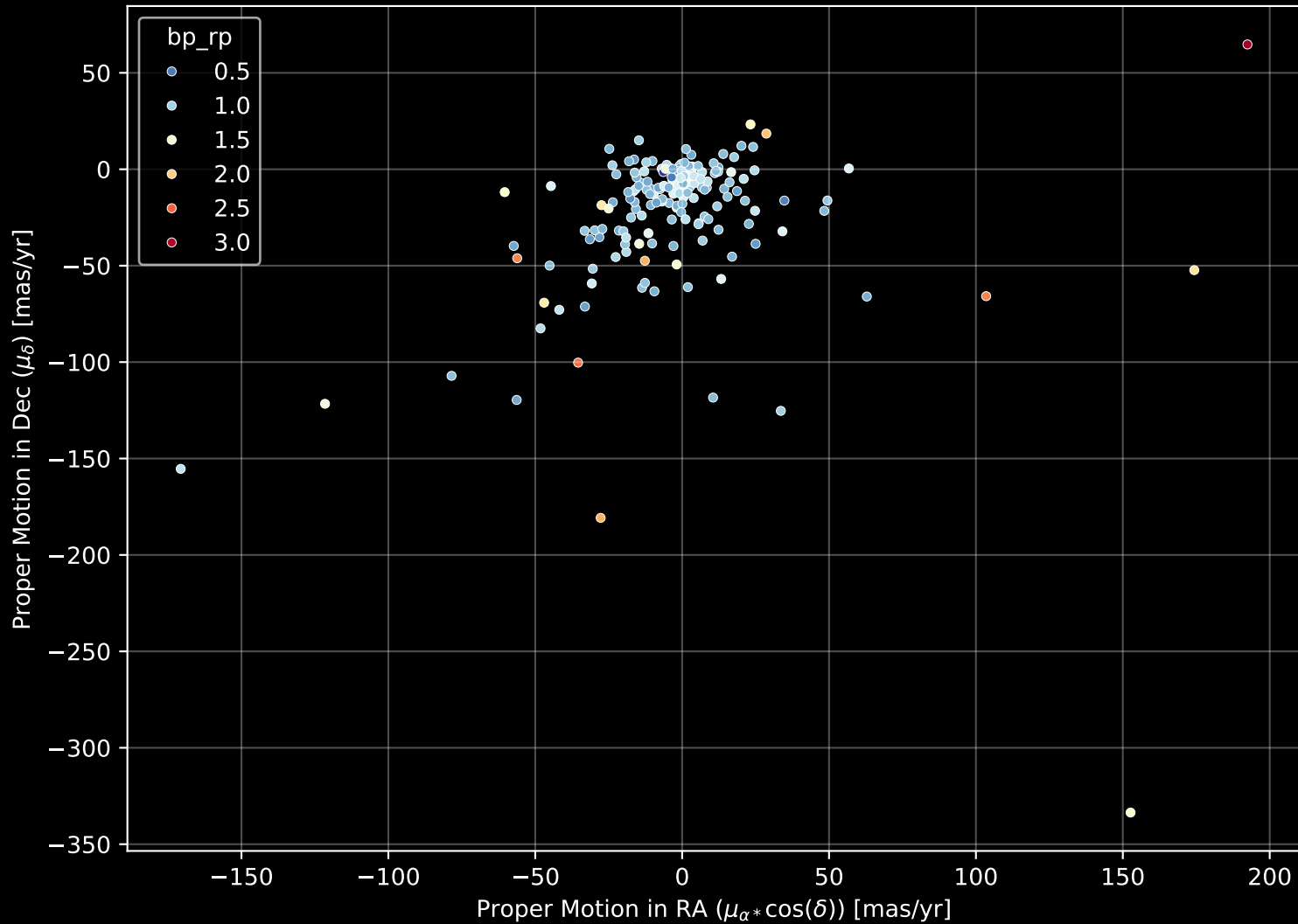
APOGEE DR17 Field: [163+36_MGA] Proper Motion Diagram (n= 205)
