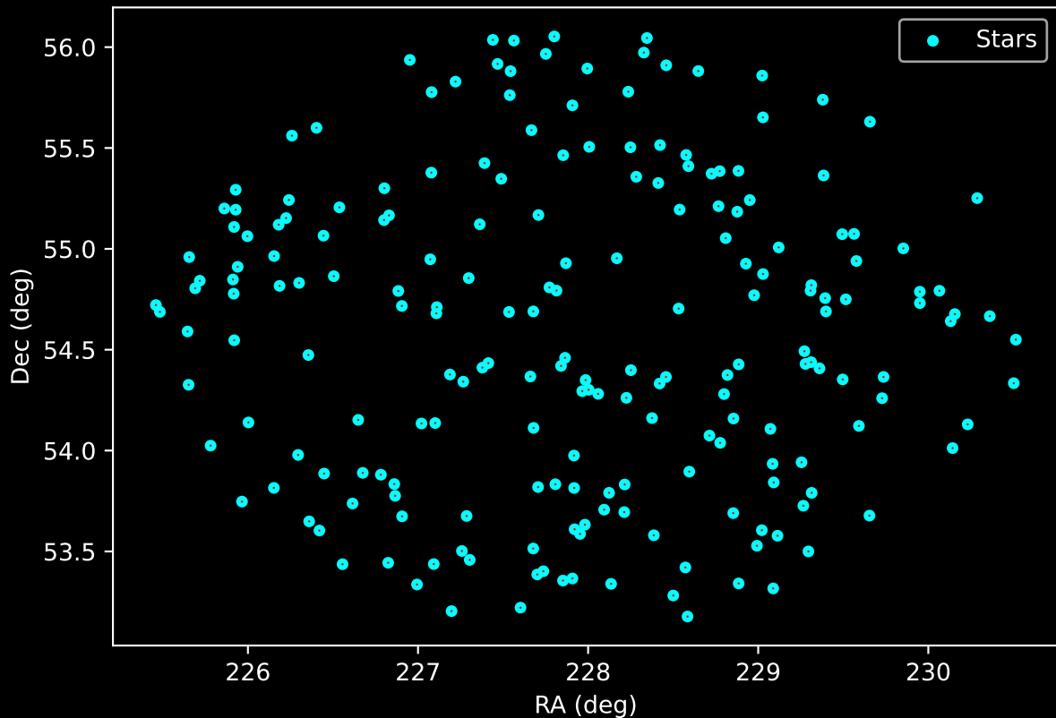
APOGEE DR17 Field: [163+36_MGA] Proper Motion Vectors for Gaia Star Field (n= 205)
