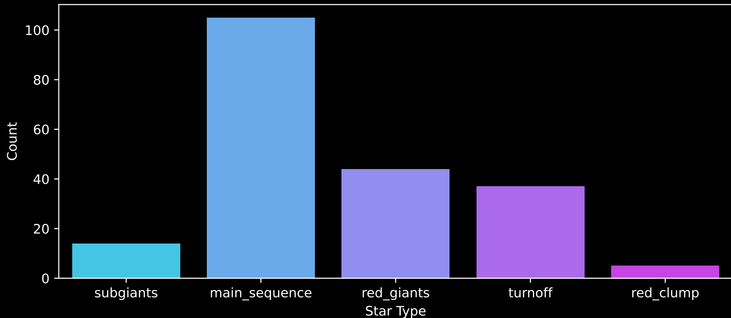
APOGEE DR17 Field: [163+36_MGA] Count plot of Star Type
