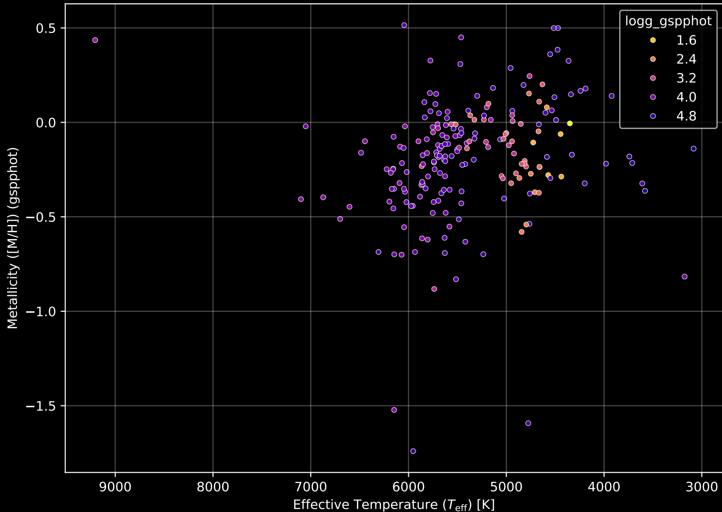
APOGEE DR17 Field: [163+36_MGA] Stellar Population Parameters (n= 205)
