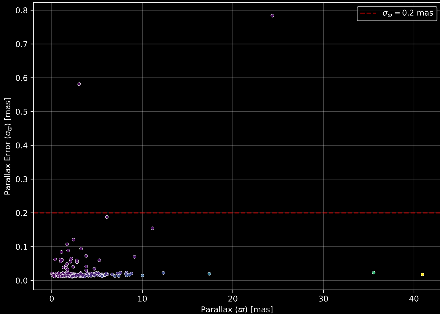
APOGEE DR17 Field: [163+36_MGA] Parallax Quality (n= 205)
