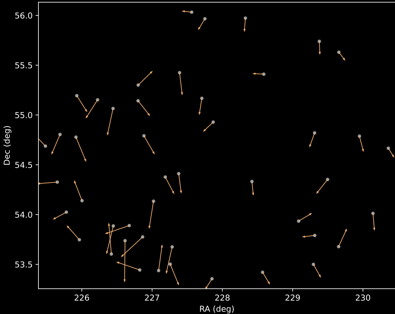
APOGEE DR17 Cluster 3 Proper Motion Vectors (n=46)
