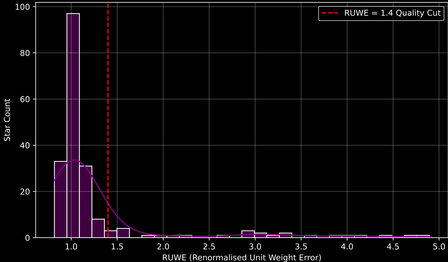
GAPOGEE DR17 Field [163+36_MGA] RUWE Distribution (n= 196)
